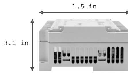
Right Side
